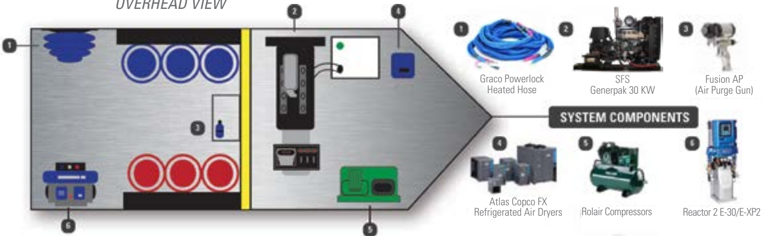
OVERHEAD VIEW
